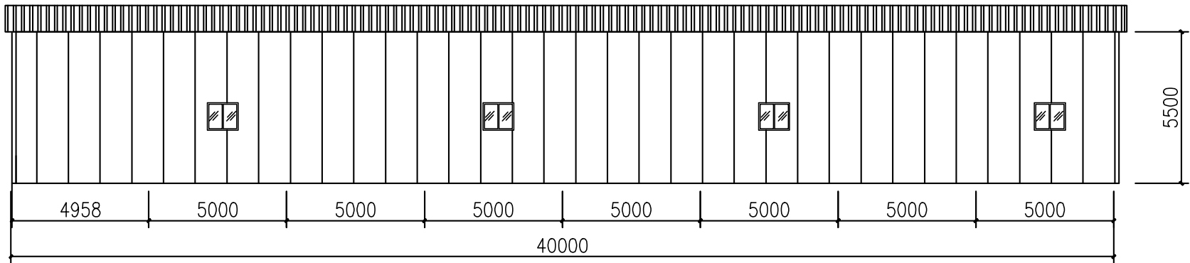
front & back elevation
