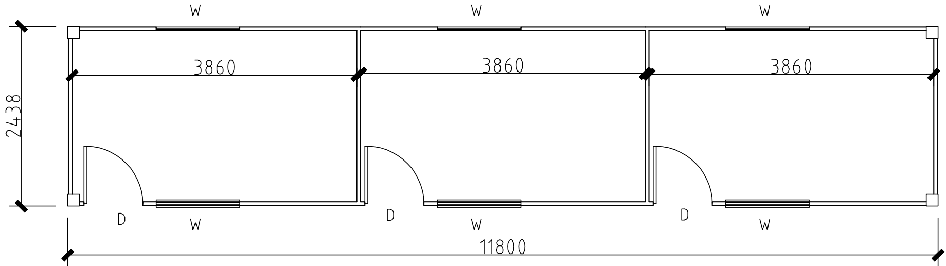
floor plan
